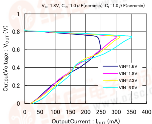
XC6415( V_{OUT}=0.8V )
