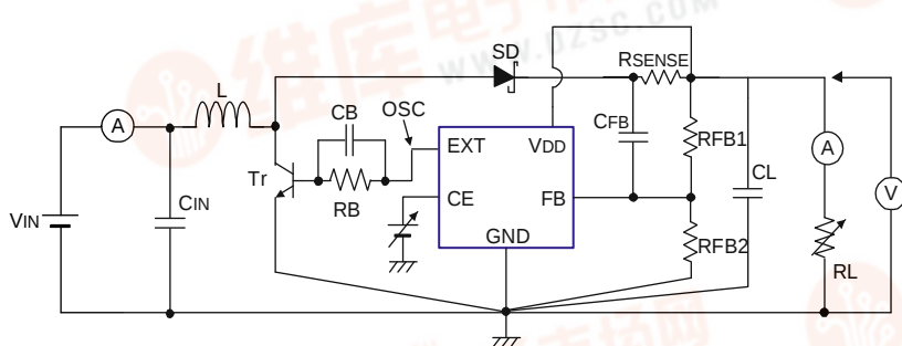
Circuit ③
