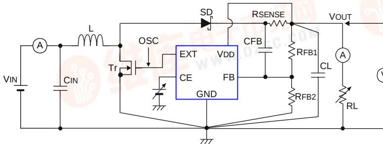
Circuit ①
