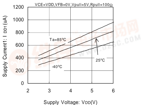
(6) Supply Current 1 vs. Supply Voltage
