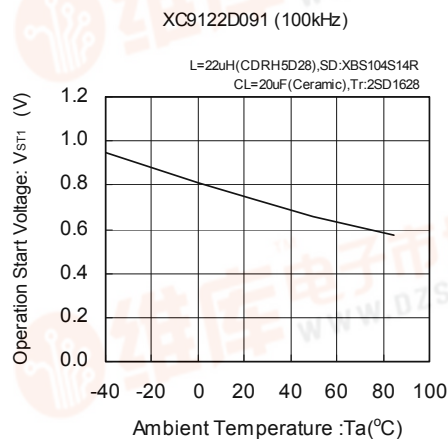
(15) Operation Start Voltage vs. Ambient Temperature
