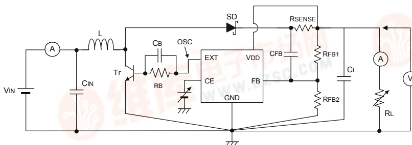
Circuit ③
