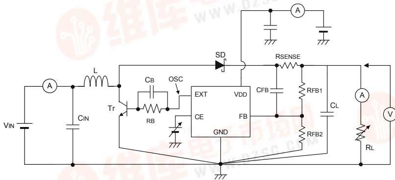
Circuit ②
