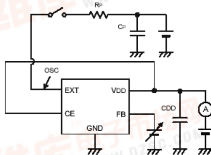
Circuit ④
