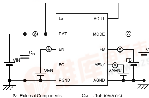
< Circuit No.2 >
