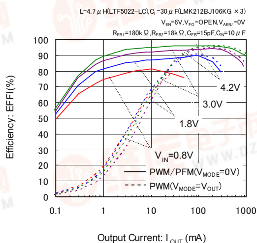
XC9128 ( V_{OUT}=5.0V )
