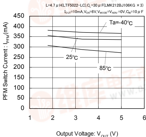
XC9128 ( V_{IN}=0.9V )
