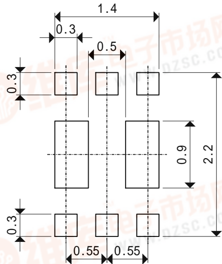
USP-6EL Reference Metal Mask Design
