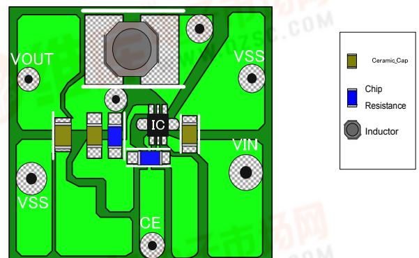
XC9235/9236/9237D, F (Output Voltage External Setting) (PKG:USP-6C)
