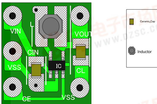
XC9235/9236/9237A, B, C (Output Voltage Fixed) (PKG:SOT-25)
