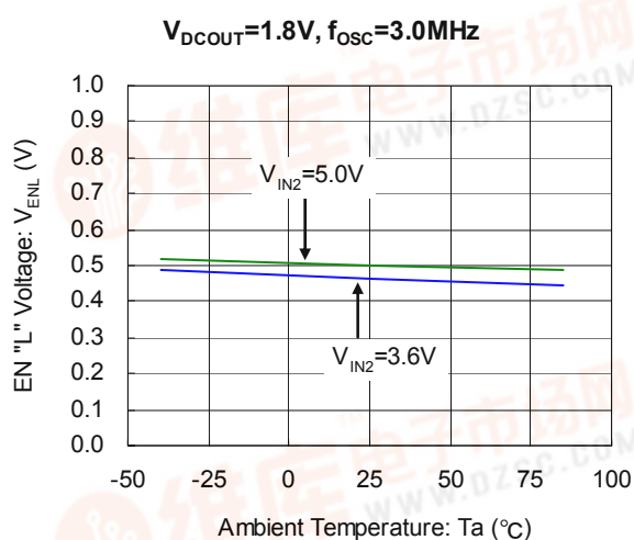
(9) EN "L" Voltage vs. Ambient Temperature
