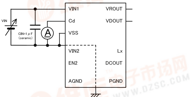
Circuit No.6
