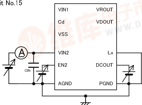
Circuit No.15
