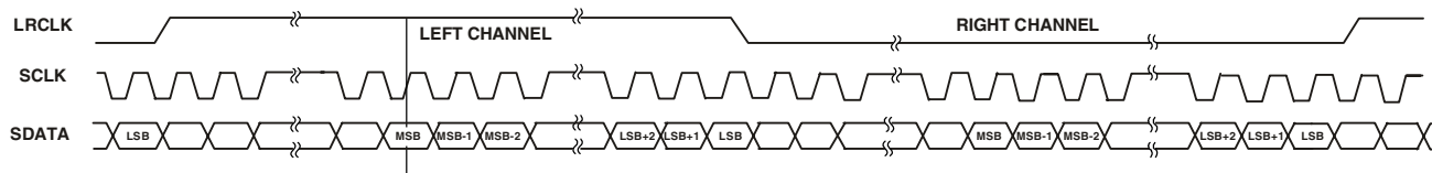
Figure 29. Right-Justified Mode
