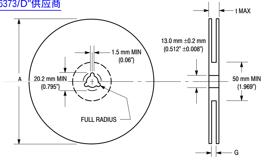
Figure 8. Reel Dimensions
