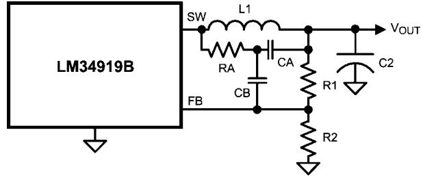
FIGURE 9. Minimum Output Ripple Using Ripple Injection
