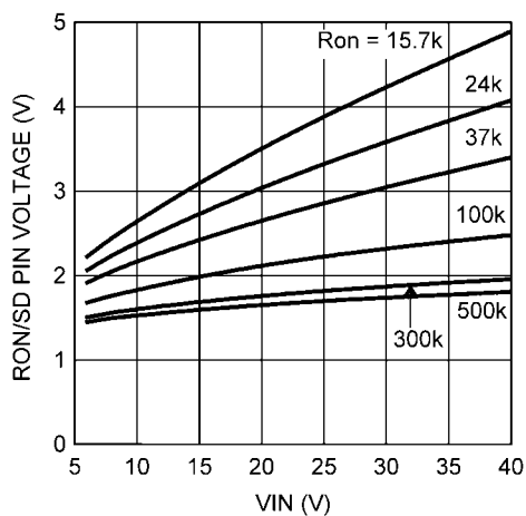
Voltage at the R_{ON}/SD Pin
