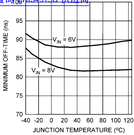
Minimum Off-Time vs. Temperature 查询"LM34919B"供应商
