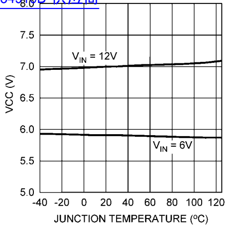
V CC Voltage vs. Temperature 查询"LM34919B"供应商
