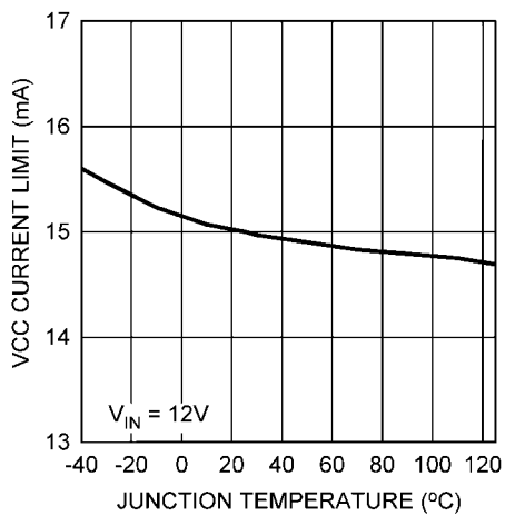
V CC Current Limit vs. Temperature
