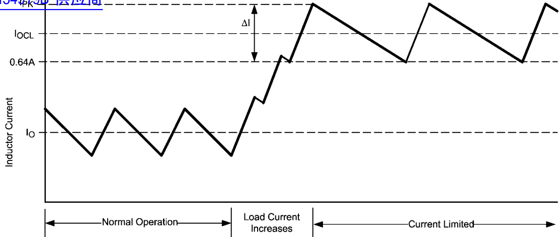
FIGURE 4. Inductor Current - Current Limit Operation
