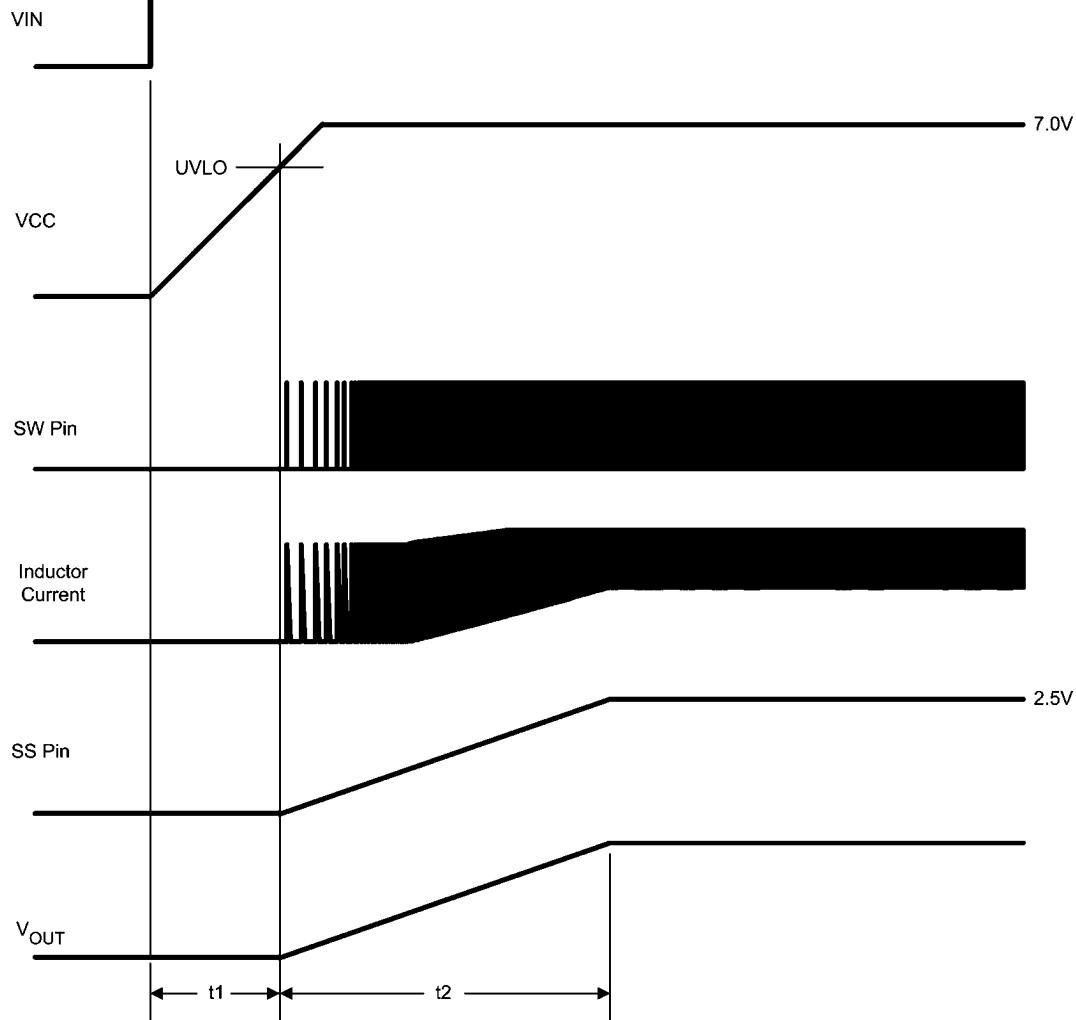
FIGURE 1. Start Up Sequence
