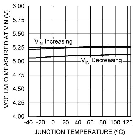
V_{CC} UVLO at V_{IN} vs. Temperature
