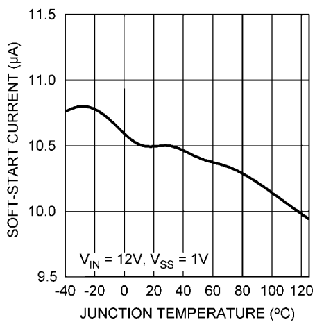
Soft-Start Current vs. Temperature
