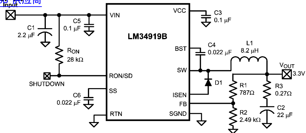
FIGURE 5. Example Circuit
