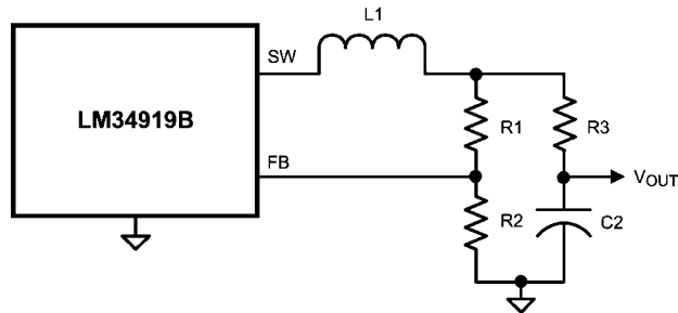
FIGURE 10. Alternate Minimum Output Ripple Configuration
