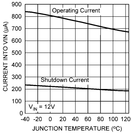
Operating &amp; Shutdown Current vs. Temperature
