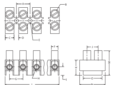
Dimensions mm
