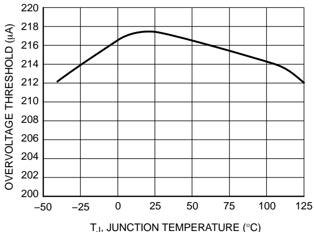
Figure 13. Overvoltage Protection Threshold vs. Temperature
