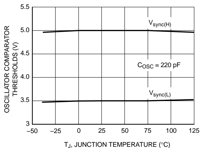
Figure 5. Oscillator Comparator Thresholds vs. Temperature
