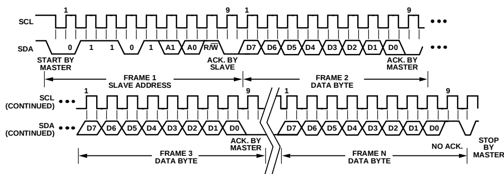
Figure 27. General SMBus Read Timing Diagram
