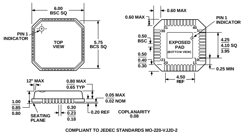
Figure 38. 40-Lead Lead Frame Chip Scale Package [LFCSFP] (CP-40) Dimensions shown in millimeters
