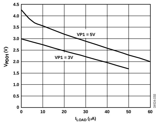
Figure 13. V_{PDO1} (Weak Pull-Up to VP ) vs. I_{LOAD}
