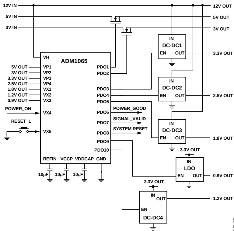
Figure 24. Applications Diagram
