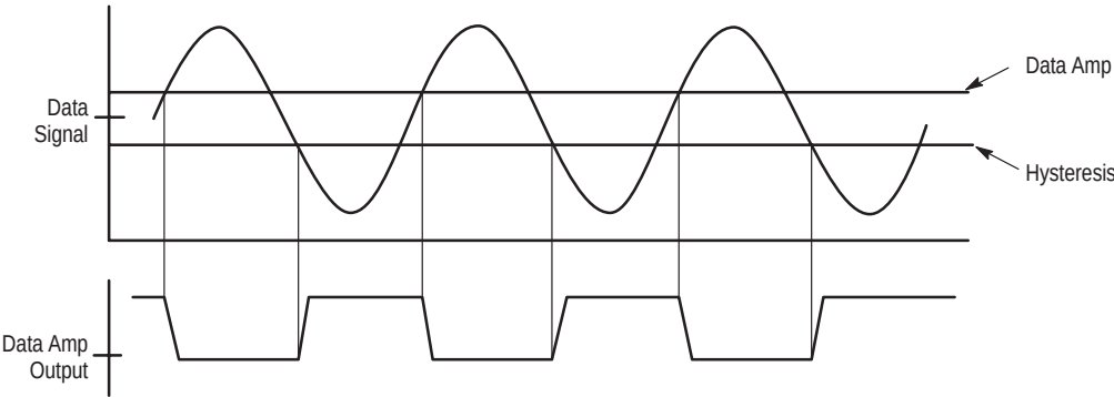
Figure 3. Data Amp Operation
