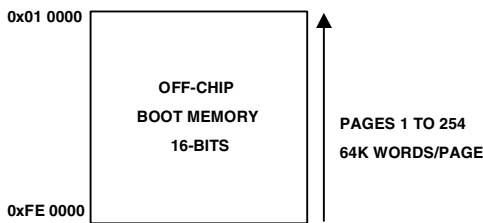
Figure 4. Boot Memory Map
