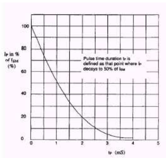
Figure 4. Pulse waveform
