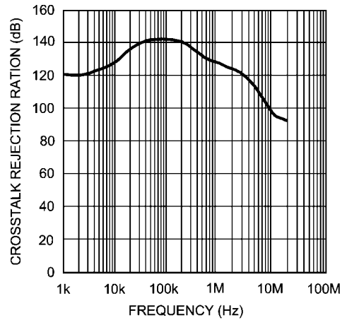
Crosstalk Rejection
