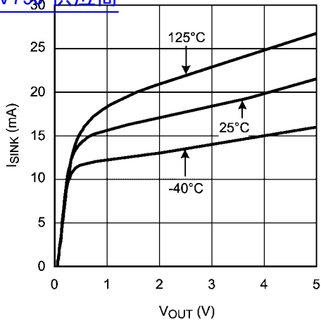
查询"LMV796"供应商 Sinking Current vs. Output Voltage
