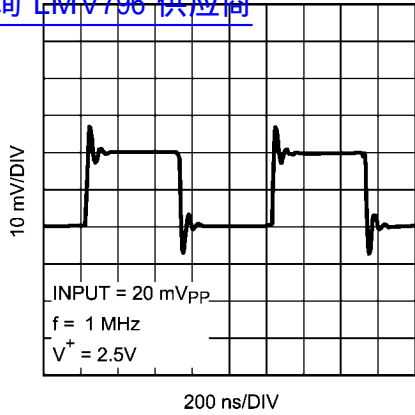
Small Signal Transient Response, A_V = +1 查询"LMV796"供应商
