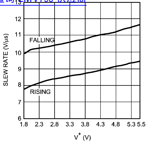
Slew Rate vs. Supply Voltage 查询"LMV796"供应商
