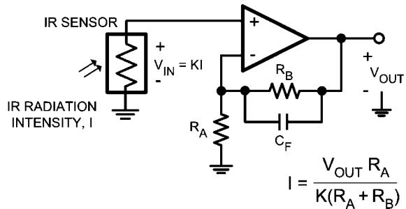
FIGURE 15. IR Radiation Sensor
