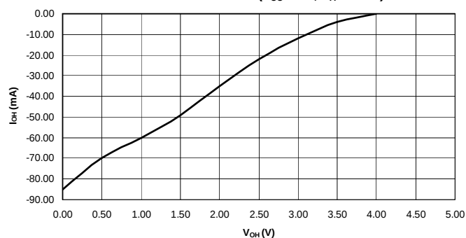
ATF750C/CL OUTPUT SOURCE CURRENT VS. OUTPUT VOLTAGE ( V_{CC} = 5\text{V} , T_A = 25^\circ\text{C} )
