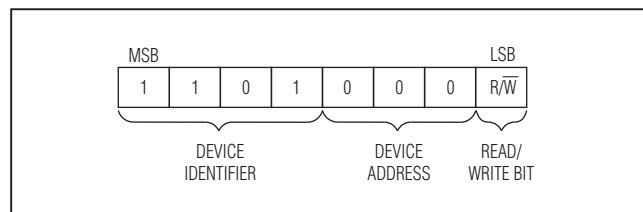
Figure 5. Slave Address Byte
