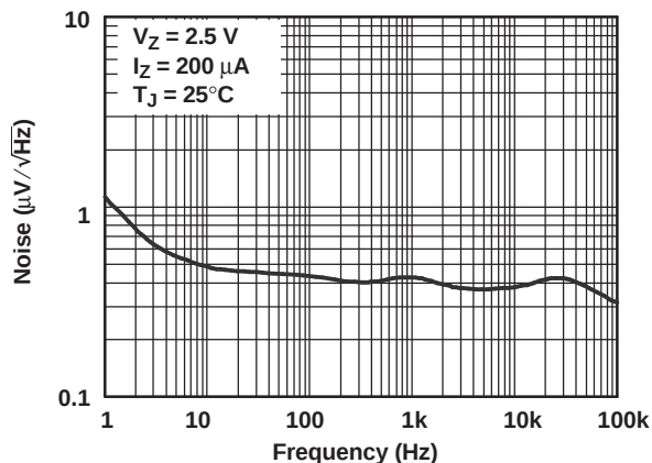
Figure 5. Noise Voltage vs Frequency
