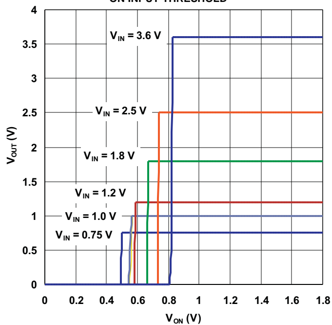
ON INPUT THRESHOLD
