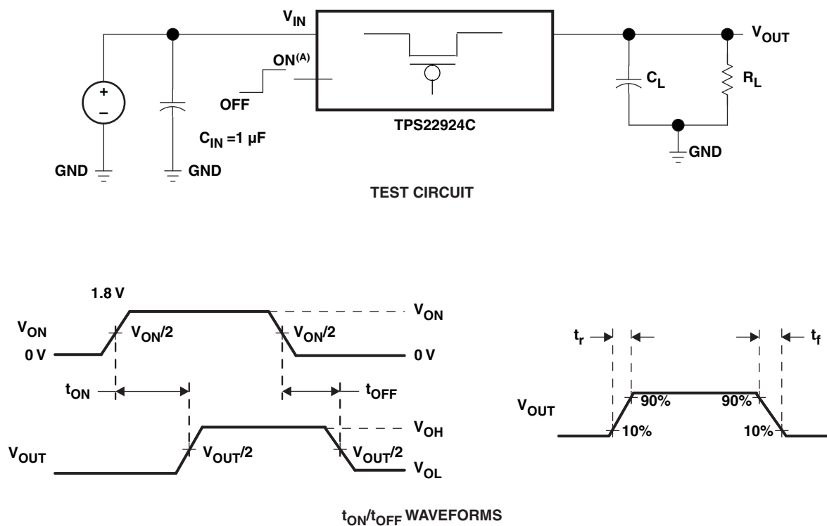
Figure 1. Test Circuit and t_{ON}/t_{OFF} Waveforms
