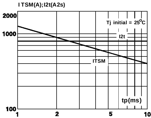
Fig. 7 : On-state repetitive surge peak on-state current for a sinusoidal pulse with width : t_p \leq 10 ms and corresponding value of I^2 t .
