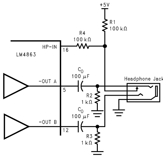
FIGURE 2. Headphone Circuit
