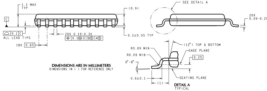
20-Lead Molded TSSOP, Exposed Pad, 6.5x4.4x0.9mm Order Number LM4863MTE NS Package Number MXA20A
