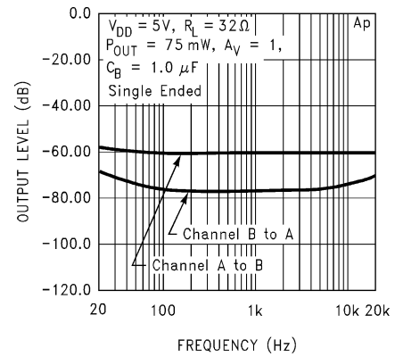
Channel Separation
