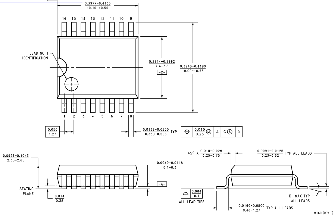
16-Lead (0.300" Wide) Molded Small Outline Package, JEDEC Order Number LM4863M NS Package Number M16B
