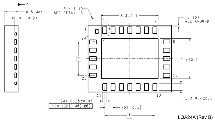
24-Lead Molded pkg, Leadframe Package LLP Order Number LM4863LQ NS Package Number LQA24A
