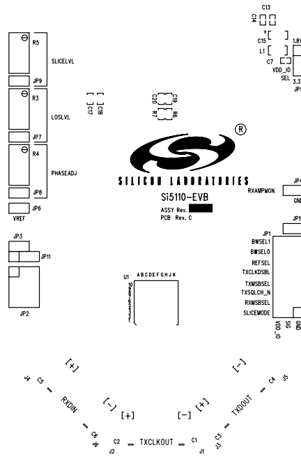
Figure 28. Si5110-EVB Component Side Assembly (Daughter Card)
