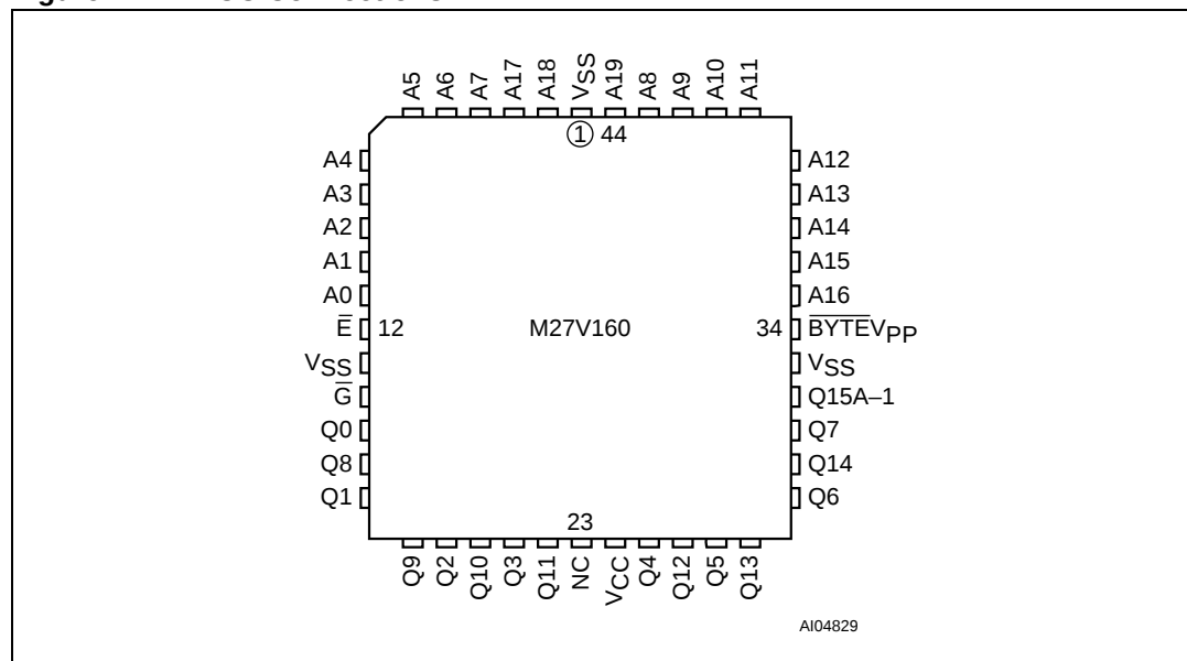
Figure 4. PLCC Connections
