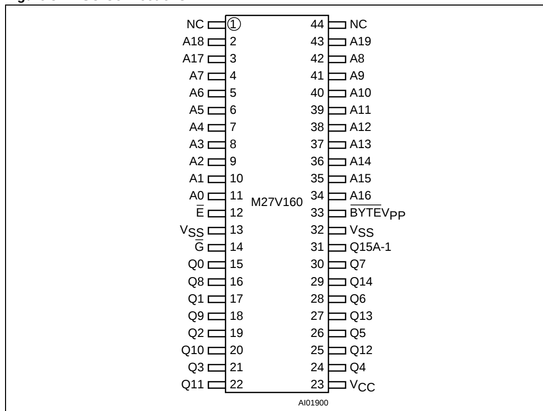
Figure 3. SO Connections
