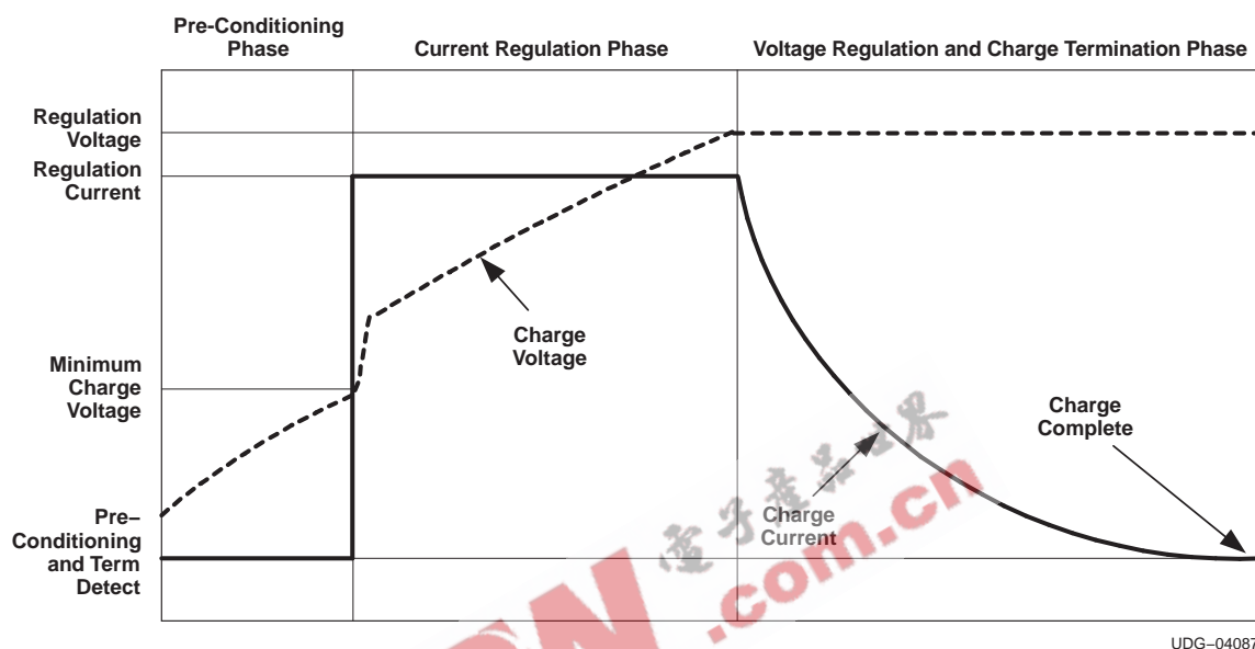
Figure 1. Charge Profile
