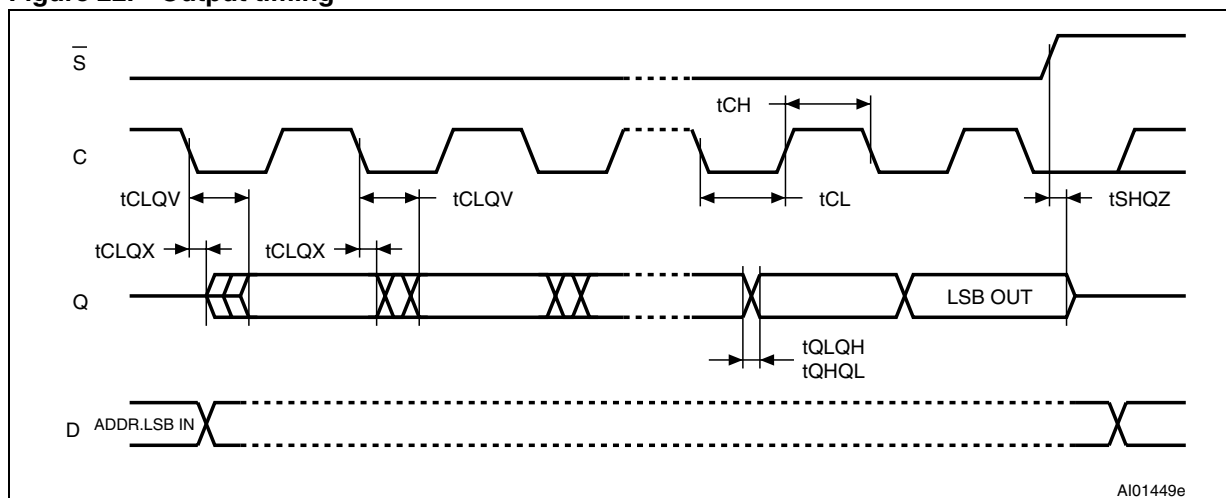
Figure 22. Output timing
