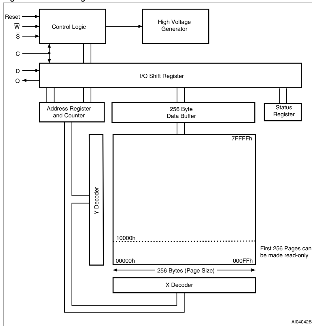
Figure 5. Block diagram
