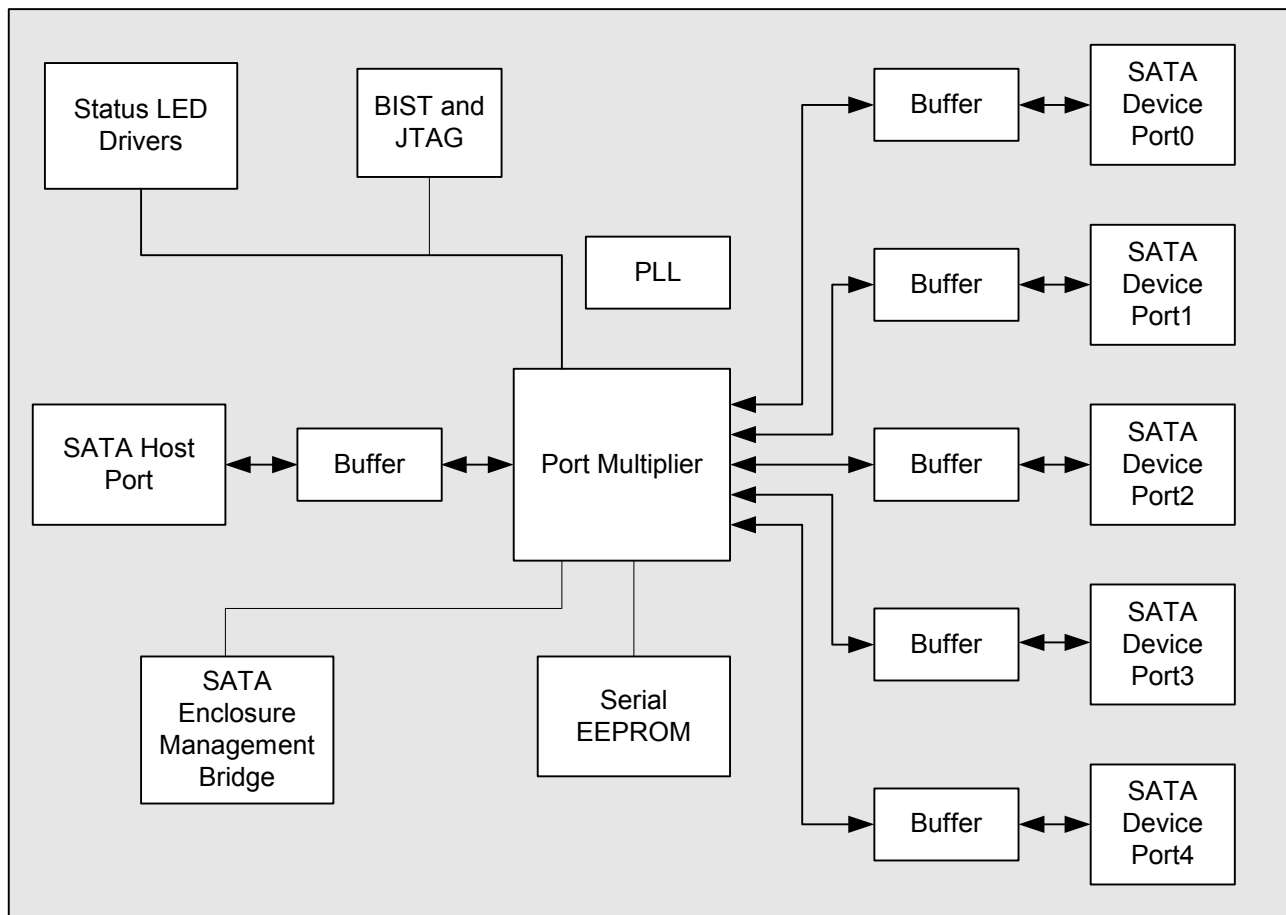
Figure 1: Sil 3726 SATA Port Multiplier Block Diagram
