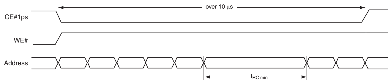
Figure 34. Read Address Skew
