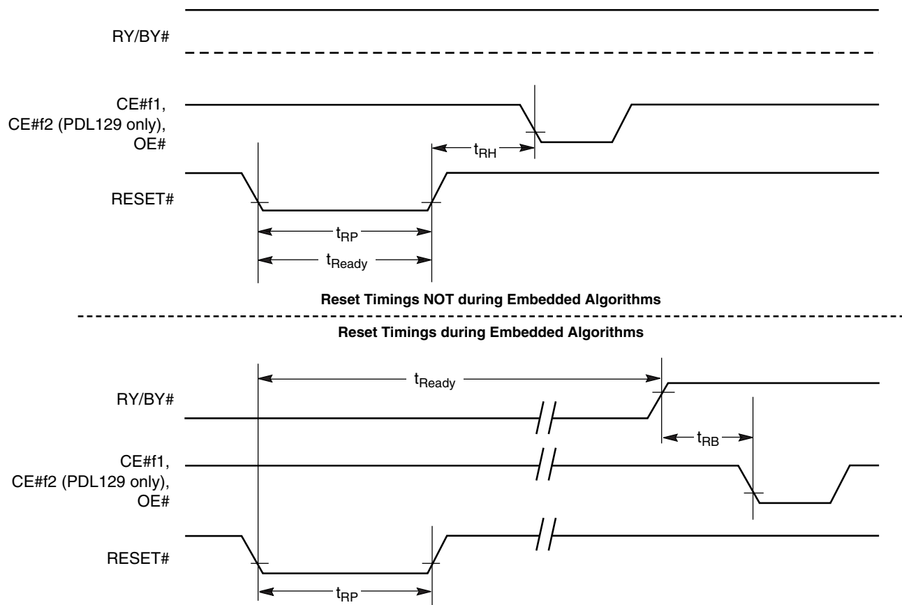
Figure 16. Reset Timings
