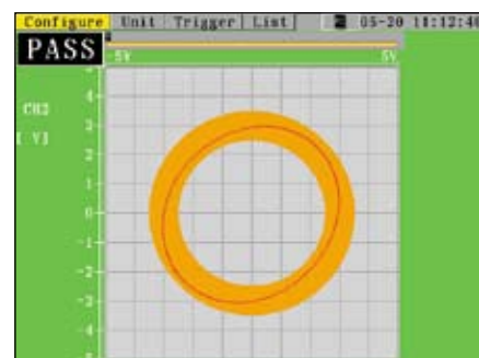
Using 2-channel input for X-Y Lissajous waveform evaluation: Vertical and horizontal voltage input allows Lissajous waveform evaluation. (Only with Model 8731-10)
