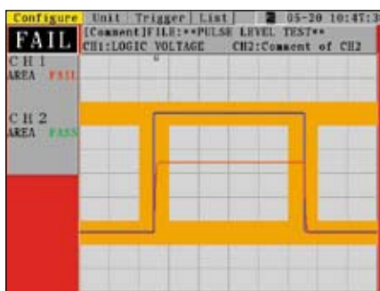
Evaluating a time axis waveform using a donut-shaped area: FAIL evaluation of a pulse with insufficient amplitude
