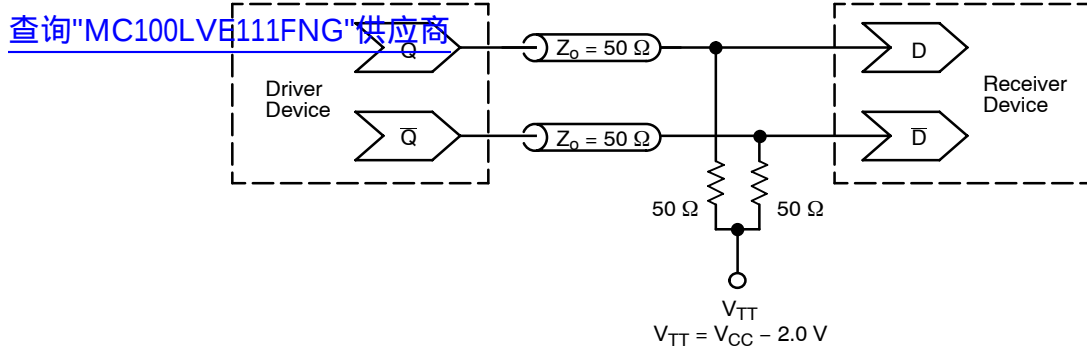
Figure 4. Typical Termination for Output Driver and Device Evaluation (See Application Note AND8020/D – Termination of ECL Logic Devices.)
