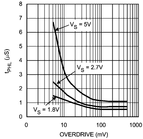
t_{PHL} vs. Overdrive
