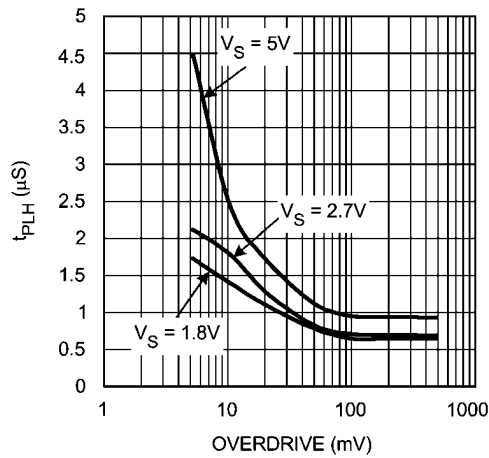
t_{PLH} vs. Overdrive
