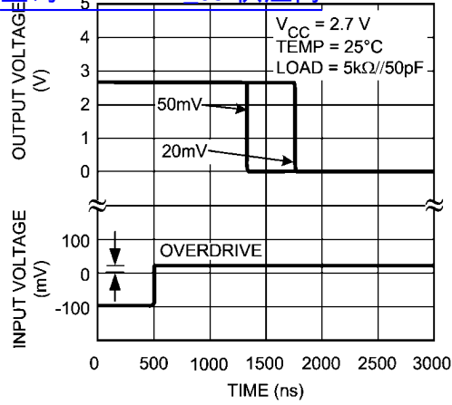
Propagation Delay ( t_{PHL} )
