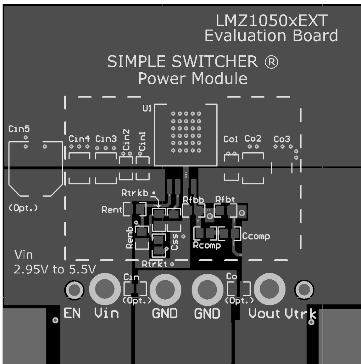
FIGURE 6. Top Copper
