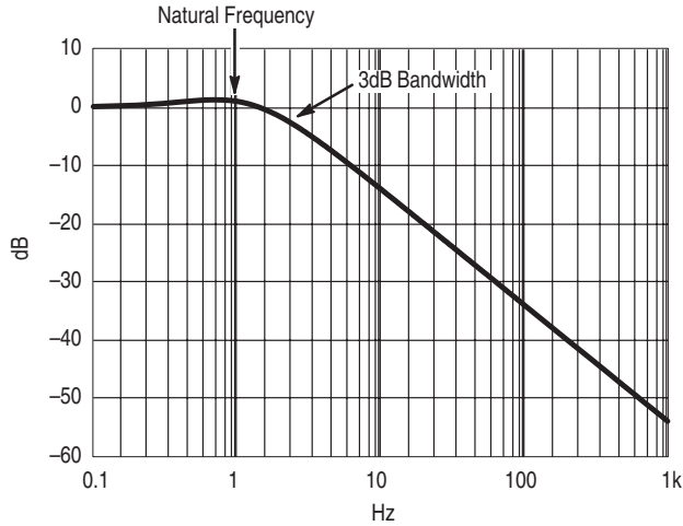
Figure 7. Closed Loop Frequency Response for \zeta = 1
