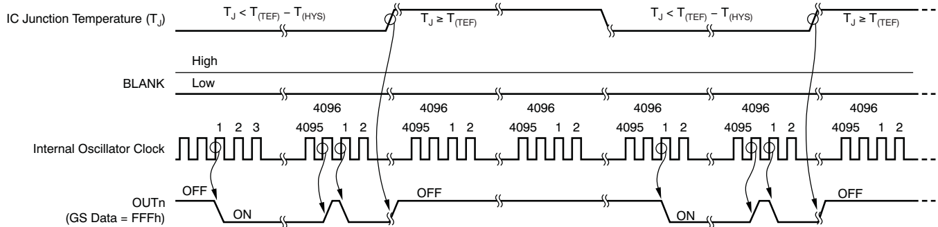
Figure 22. TSD Operation
