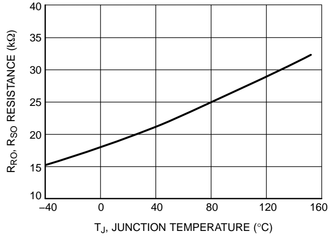
Figure 38. R RO , R SO Resistance vs. Junction Temperature
