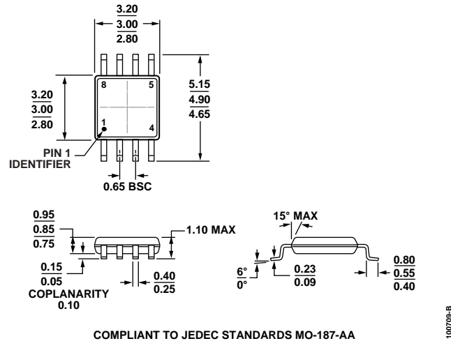
COMPLIANT TO JEDEC STANDARDS MO-187-AA Figure 28. 8-Lead Mini Small Outline Package [MSOP] (RM-8) Dimensions shown in millimeters
