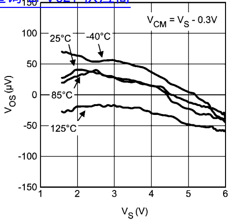
Input Offset Voltage vs. Supply Voltage 查询"LPV521"供应商
