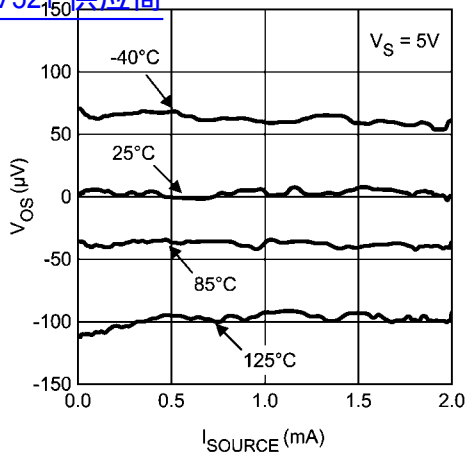
Input Offset Voltage vs. Sourcing Current 查询"LPV521"供应商
