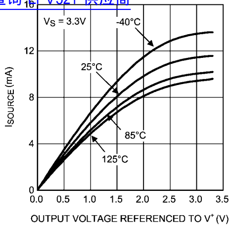
Sourcing Current vs. Output Voltage 查询"LPV521"供应商
