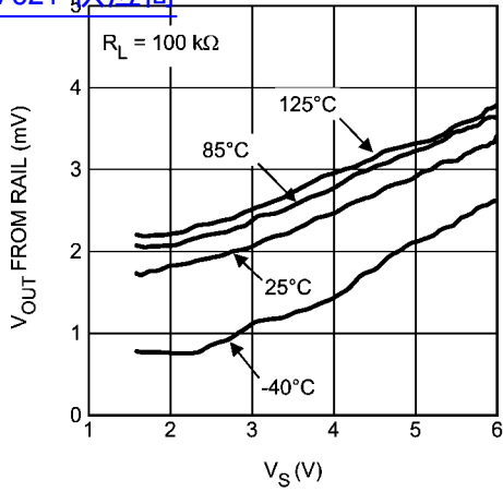
Output Swing High vs. Supply Voltage 查询"LPV521"供应商
