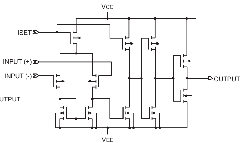
Comparator
