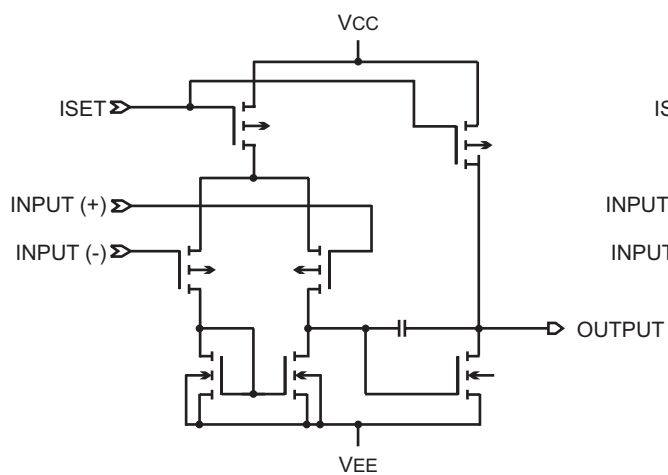
Operational Amplifier
