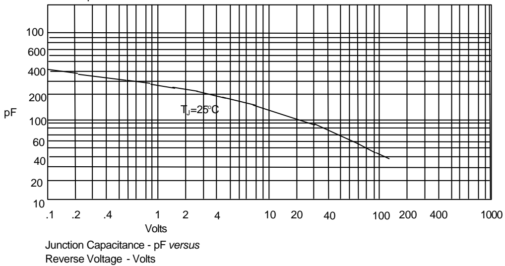
Figure 3 Junction Capacitance
