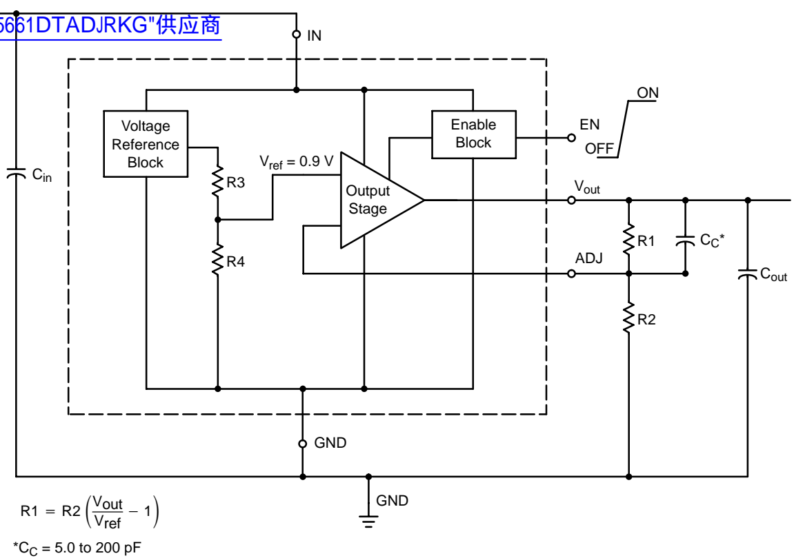
Figure 1. Typical Schematic, Adjustable Output Version
