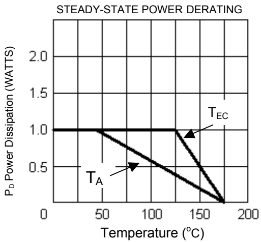
FIGURE 1 Power Derating Curve Where T_{EC} is End Cap Temp and T_A is Ambient Temperature on FR4 PC board.
