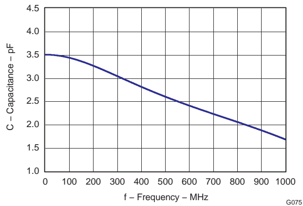
Figure 95. ADC Analog Input Capacitance (Cin) Across Frequency
