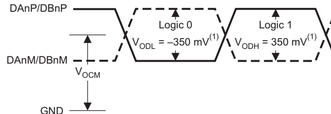
Figure 3. LVDS Output Voltage Levels
