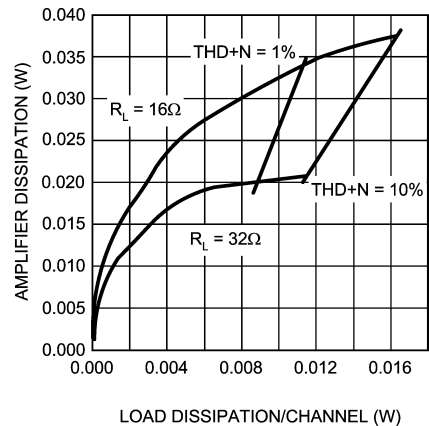
Load Dissipation vs Amplifier Dissipation
