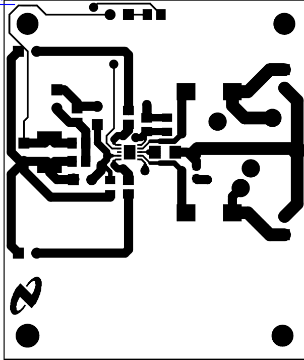
FIGURE 6. Top Layer
