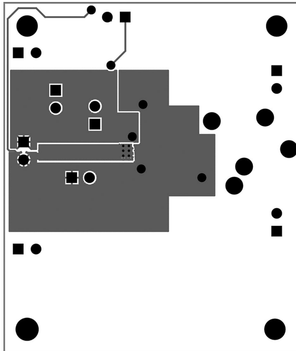
FIGURE 7. Bottom Layer
