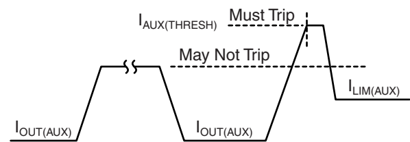
Figure 4. VAUX Current Limit Threshold
