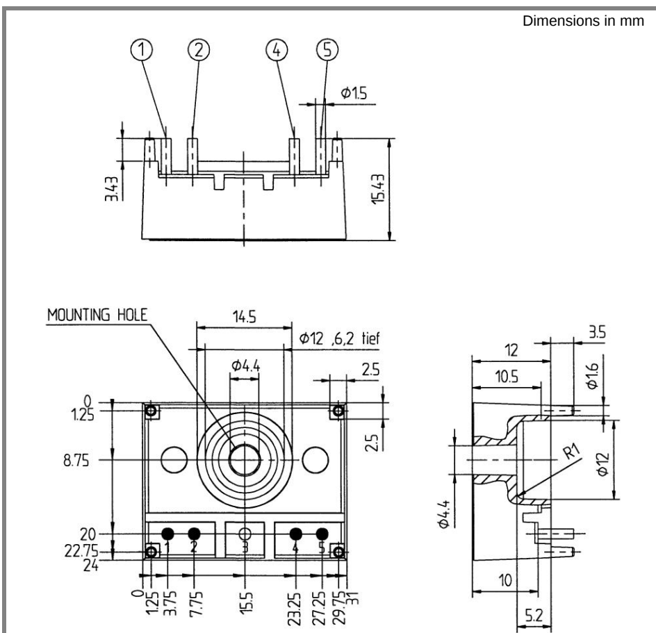
Case T 1 (Suggested hole diameter in the PCB for solder pins and mounting pins : 2mm)
