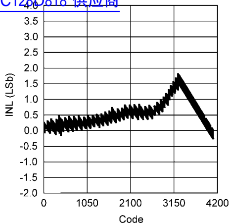
INL vs. Code (External VREF = 2.56V for 1 Unit) 查询"ADC128D818"供应商
