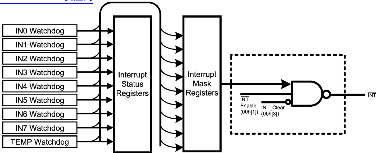
FIGURE 13. Interrupt Structure
