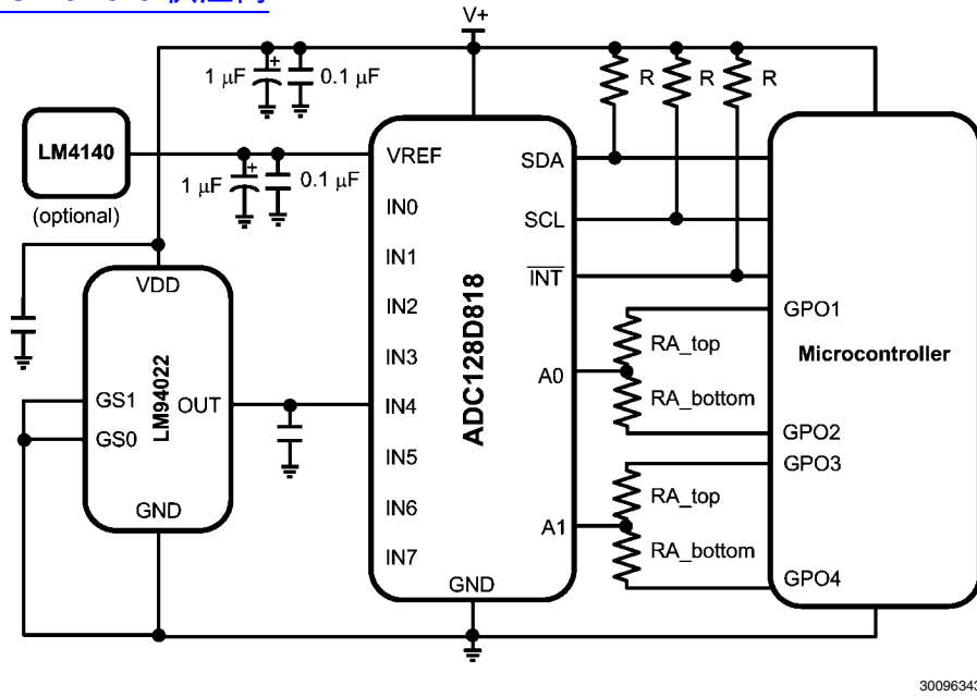
FIGURE 17. Temperature Sensor Applications
