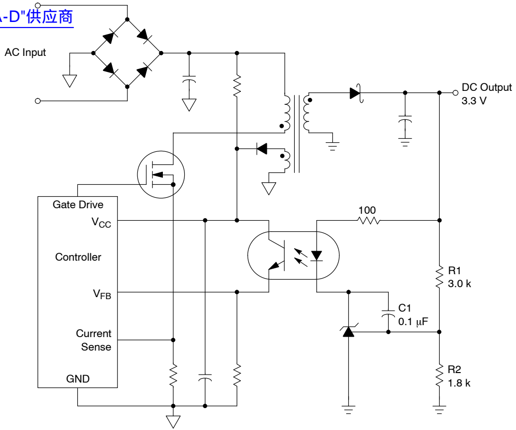
Figure 31. Isolated Output Line Powered Switching Power Supply
