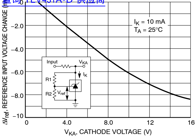
Figure 10. Reference Input Voltage Change versus Cathode Voltage
